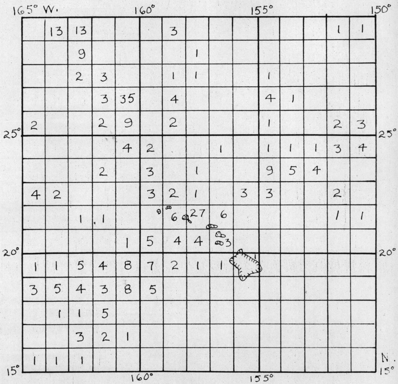
DISTRIBUTION OF BATHYTHERMOGRAPH OBSERVATIONS DECEMBER
