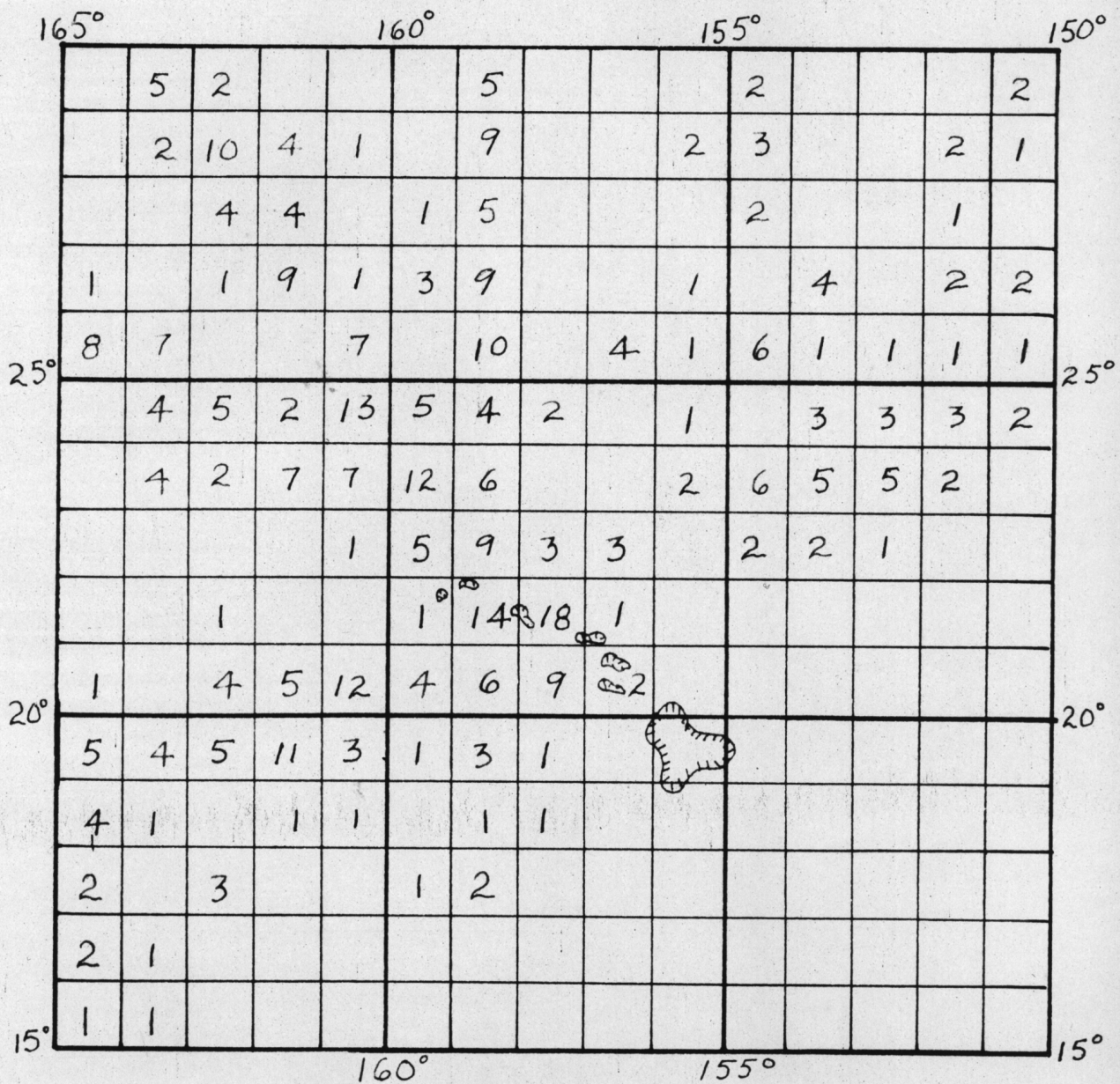
DISTRIBUTION OF BATHYTHERMOGRAPH OBSERVATIONS SEPTEMBER
