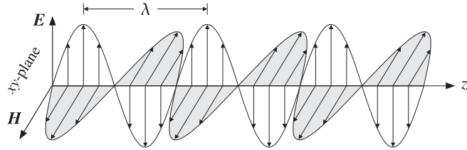
Fig. 2.2.1 Forward uniform plane wave.
